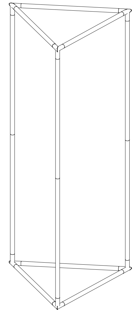
Completed Assembly
